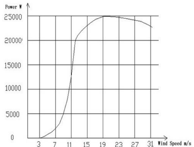
20KW power curve
