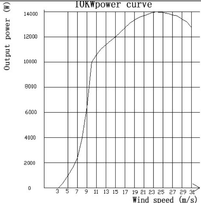
10KWpower curve
